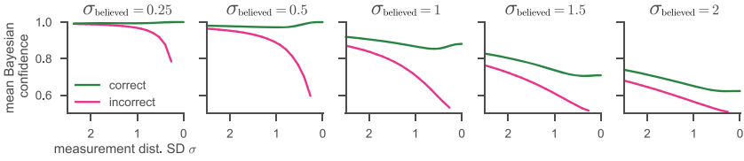
Figure 8: As in Figure 4c. True measurement noise is \sigma = 1 . Divergence signature 2 is not present or is present only weakly.
